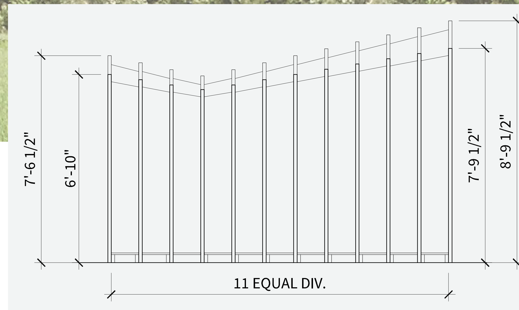
Side Elevation
